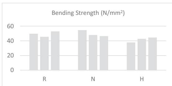
Figure 8: Bending strength – all panels
