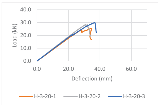
Figure 5: Load-deflection response – hybrid timber panels
