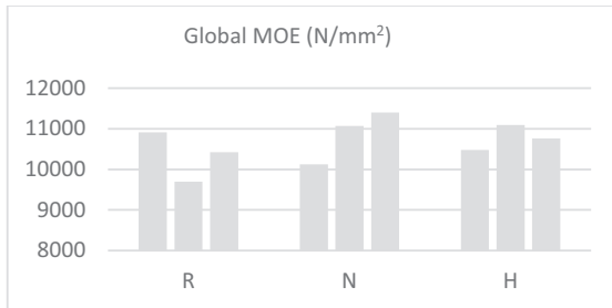
Figure 7: Global Modulus of elasticity – all panels
