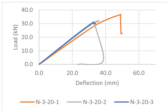
Figure 4: Load-deflection response – new timber panels
