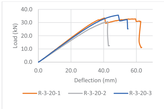
Figure 3: Load-deflection response – recovered timber panels
